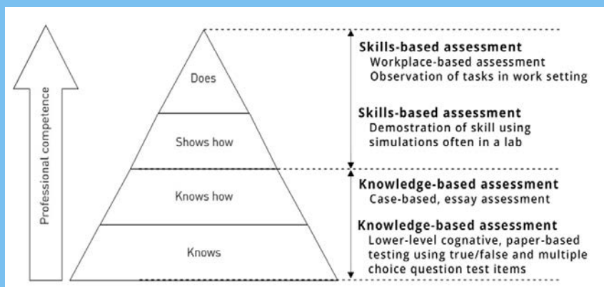
Figure 1: Miller's pyramid
